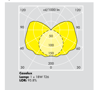
Opal diffuser
