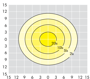
Plurio with faceted reflector and clear bowl Lamp: 70W HIE DLOR: 69% ULOR: 1%
