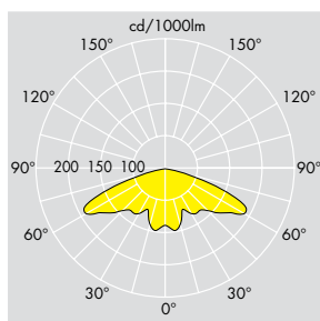
Plurio with faceted reflector and clear bowl Lamp: 70W HIE DLOR: 69% ULOR: 1%
