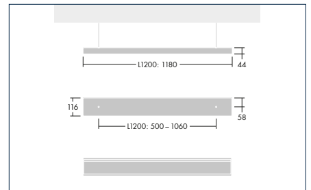
PUNCH ASYMMETRIC
