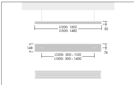
PUNCH SUSPENDED
